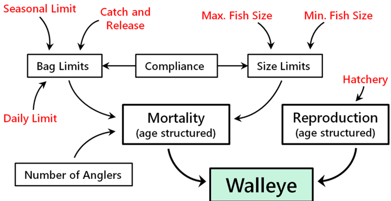
Fig. 11.25. The conceptual model of walleye population dynamics used to support recovery planning. The items in red represent management levers that were explored in stakeholder workshops.
