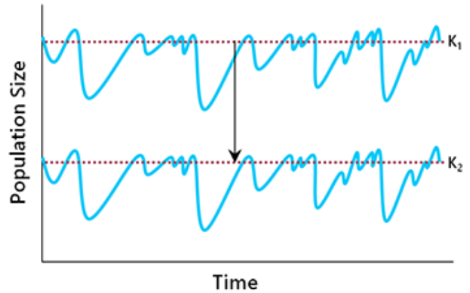
Fig. 6.6. When K is reduced, the population will equilibrate at a lower density, potentially exposing it to the demographic challenges of small populations.
