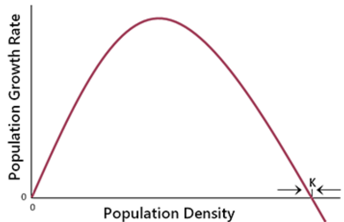
Fig. 6.2. Population growth rate as a function of population density, given the functional relationships shown in Fig. 6.1.
