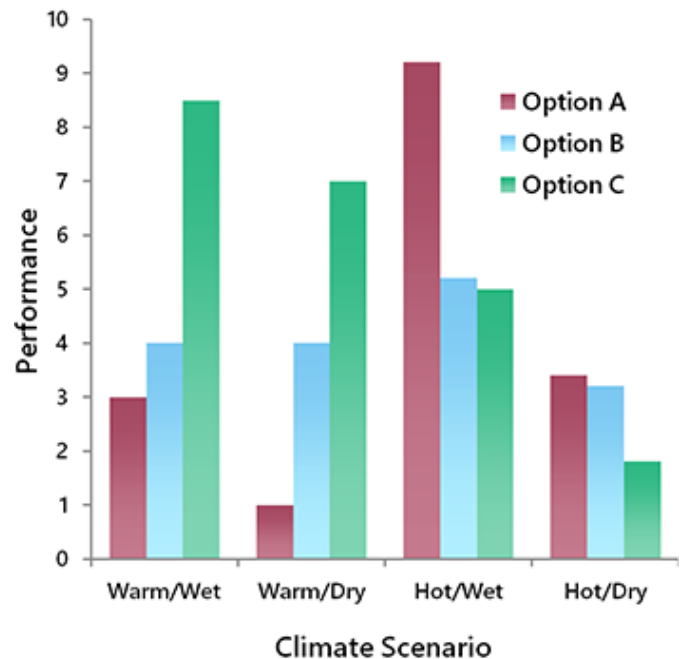
Fig. 9.11. A hypothetical example illustrating the long-term performance of three management options under four climate scenarios. Option A achieves the highest performance, but only if the climate is hot and wet. Option B provides the most consistent performance. Option C delivers the best mean performance.
