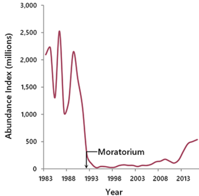
Fig. 6.8. The abundance of northern cod, 1983–2016, from autumn surveys. Stock levels remained collapsed for 20 years despite a moratorium on commercial harvesting implemented in 1992, but are now beginning to recover. Source: FOC 2017b.
