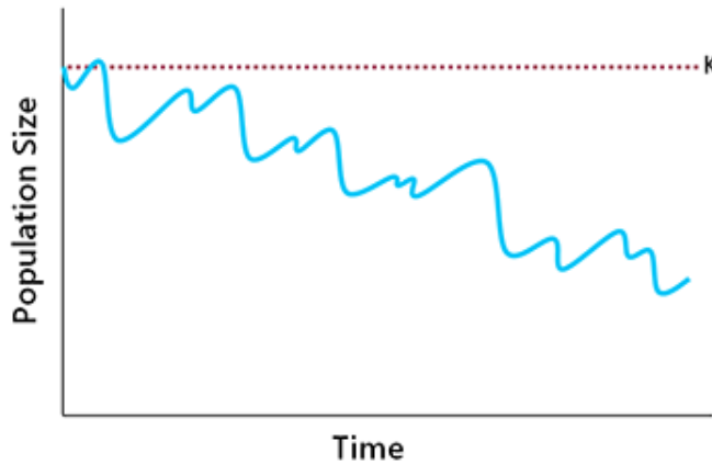
Fig. 6.5. If a population's intrinsic growth rate declines, it may be unable to recover quickly enough from periodic environmental disturbances to prevent a declining trend.
