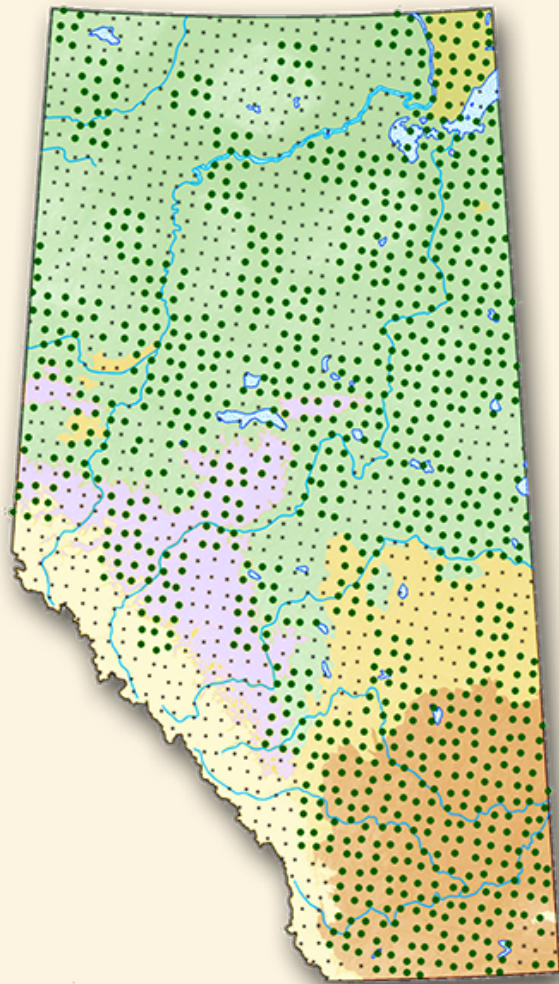
Fig. 10.9. The ABMI survey grid. The larger green circles have been sampled at least once (as of 2016) and the smaller grey points are awaiting their first visit. Source: ABMI.
