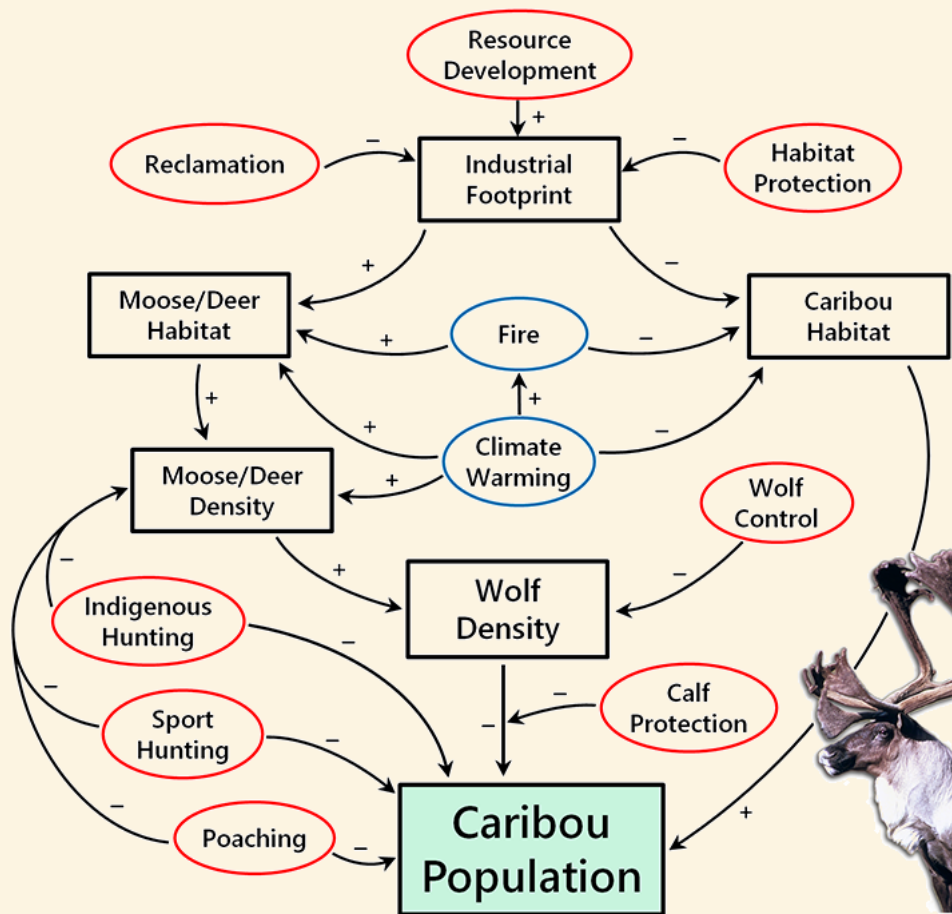
Fig. 10.4. A conceptual model illustrating the effects of management actions on woodland caribou populations. Stock variables are shown in black squares, flow variables for management actions are shown in red ovals, and external flow variables are shown in blue ovals. Plus and minus signs indicate a net positive or negative relationship. This model is a synthesis based largely on federal and provincial caribou recovery plans. Photo credit: J. Nickles.
