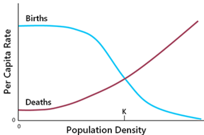
Fig. 6.1. Per capita birth rate and death rate as a function of population density, illustrating simple density-dependent relationships.
