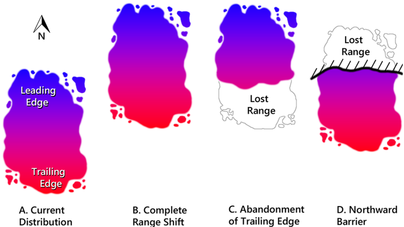
Fig. 9.16. Many species exhibit genetic adaptations to local climatic conditions, illustrated here in a red (warm) to blue (cool) colour spectrum. Panel A represents the current distribution of a hypothetical species. Panel B represents its future distribution under a warmer climate, assuming that the range shift is not impeded and all genetic variation is maintained. Panel C illustrates the future distribution that may arise if trailing-edge populations are allowed to become extirpated. The range has contracted because the gene pool is smaller and cannot accommodate the same spectrum of environmental conditions. Panel D illustrates an alternate scenario in which a barrier prevents the species from shifting its range northward. The species remains viable because warm-adapted populations replace cool-adapted populations, but the range is compressed.
