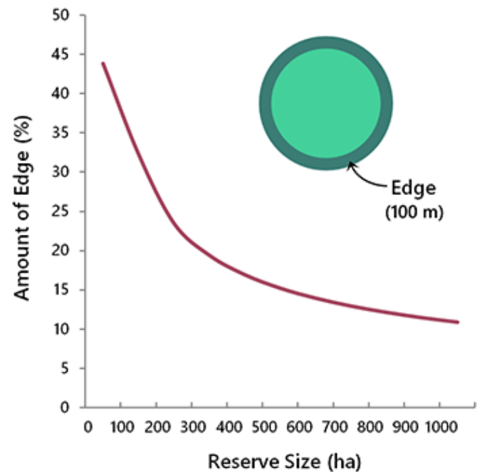
Fig. 8.6. Edge effects are a major concern for small reserves. This graph illustrates the percentage of a reserve affected by edge effects as a function of reserve size, given edge effects that extend 100 m into the reserve.
