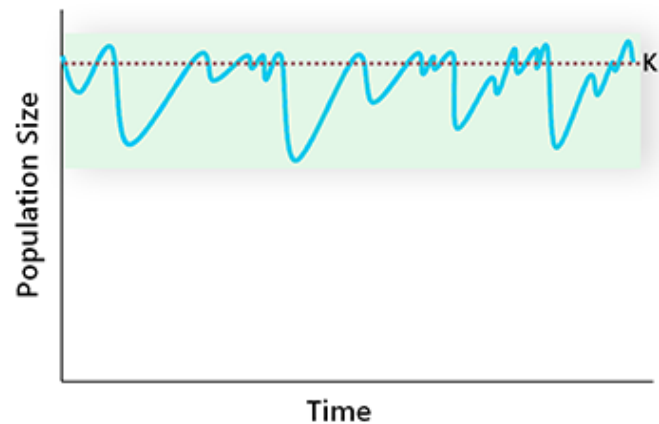
Fig. 6.3. Natural populations (blue line) fluctuate about their equilibrium level K (dotted red line) as a result of periodic environmental disturbances. The shaded area corresponds to the NRV.
