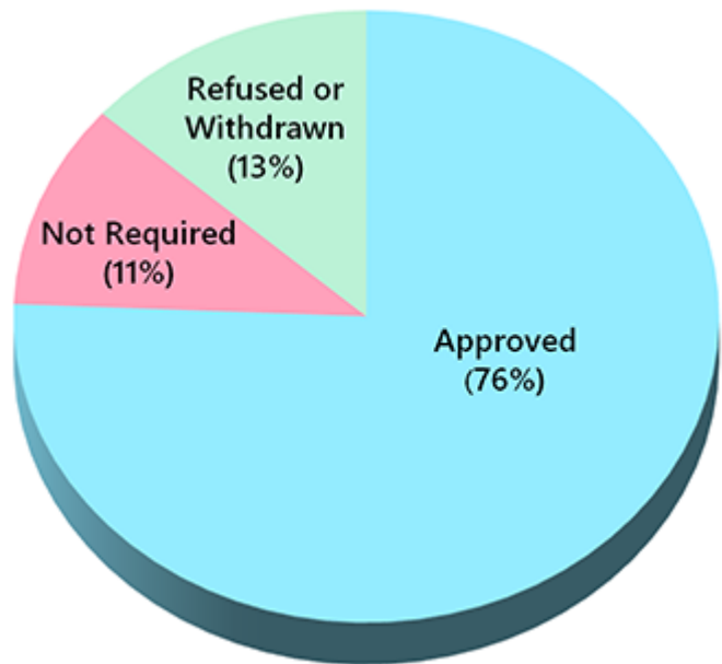
Fig. 7.14. The outcomes of environmental assessments in BC, 1992-2012 (n=156; BCEAO 2012).
