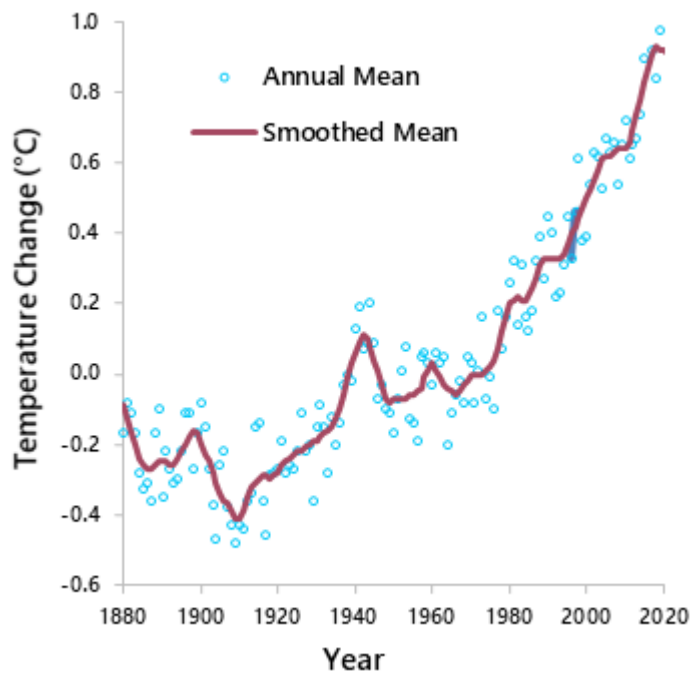
Fig. 9.1. The change in global surface temperature from 1880–2022, relative to the 1951–1980 reference period. Source: NASA 2023.
