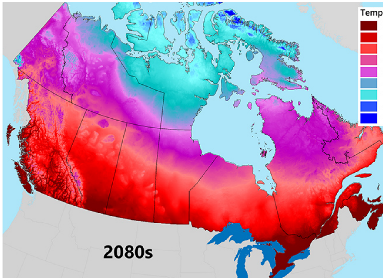
Fig. 9.3. The mean annual temperature in Canada. Top: 1961–1990 reference period. Bottom: projected temperature under the second-lowest emission scenario (RCP 4.5; ensemble mean). Source: ClimateNA interpolation, available at https://adaptwest.databasin.org/pages/adaptwest-climatena .
