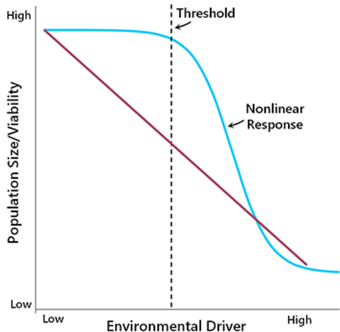
Fig. 6.7. Hypothetical response curves to an environmental driver illustrating linear and non-linear relationships. The ecological threshold, applicable to the nonlinear curve, is also shown.
