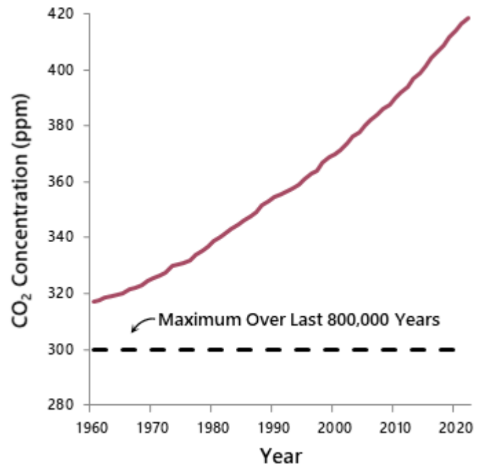
Fig. 9.2. Global CO 2 concentration, 1960–2022. The dashed line indicates the maximum CO 2 level recorded over the preceding 800,000 years. Source: Lüthi et al. 2008; NASA 2023.
