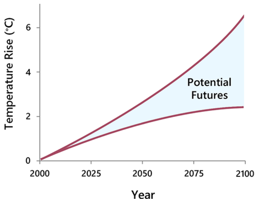
Fig. 9.10. The range of potential future climates diverges significantly in the latter half of the century because emission scenarios become more distinct and climate modeling uncertainties increase. Adapted from Schneider 2013.
