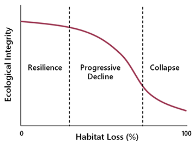
Fig. 8.4. The relationship between habitat loss and ecological integrity is nonlinear. In most applications, the shape of the curve can only be described qualitatively, as shown in this graph.
