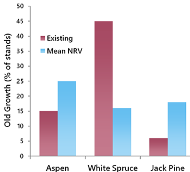
Fig. 11.3. The existing amount of old-growth on the Al-Pac FMA (red), and the predicted long-term average amount of old-growth on the FMA based on a burn rate of 1.3% per year (blue), by stand type. Source: Al-Pac 2007.
