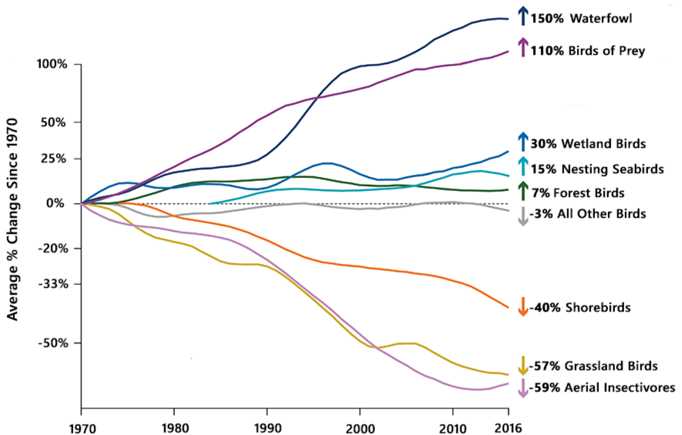
Fig. 5.1. The average change in population size since 1970, by bird group (NABCI 2019.)
