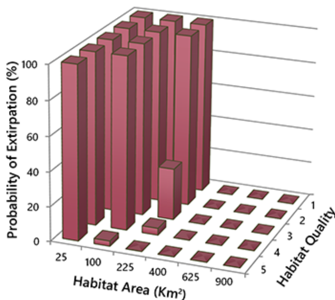
Fig. 6.13. Population viability analysis results for the threatened Newfoundland marten population. The results illustrate the effect of habitat area and quality on the probability of marten extirpation. Adapted from Schneider and Yodzis 1994.
