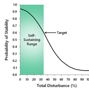
Fig. 11.14. The data presented in Fig. 11.13 can be used to show the probability of herd stability as a function of range-wide disturbance. The caribou recovery team equated critical habitat with a requirement to achieve a minimum 0.6 probability of herd stability (i.e., 60%). This threshold corresponded to a maximum 35% disturbance of the range (i.e., 65% undisturbed). Adapted from EC 2012c.
