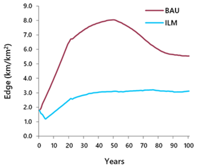
Fig. 11.4. ALCES model projections of the level of disturbance on the Al-Pac FMA over the next 100 years, measured in terms of the density of forest edge habitat resulting from roads, seismic lines, wells, pipelines, and harvest blocks. BAU = business as usual; ILM = integrated landscape management. Source: Schneider et al. 2003.
